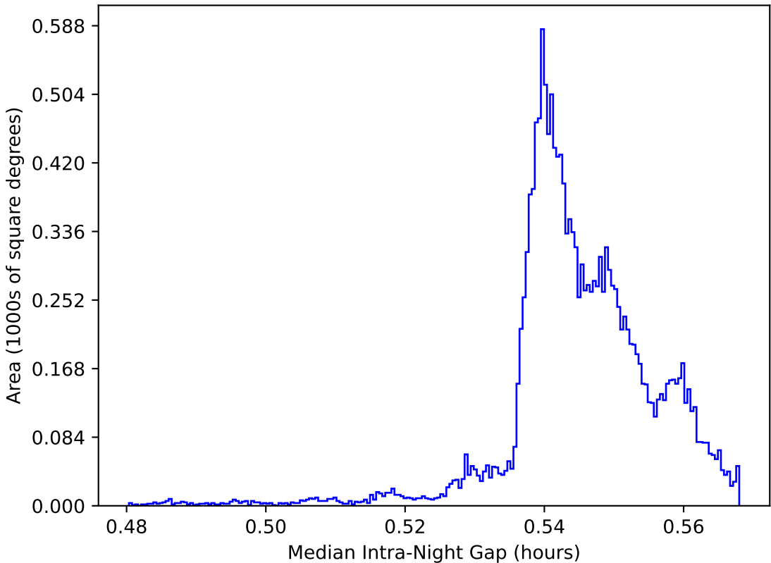
too_elab_r32_d2_griz_v3.4_10yrs WFD: Median Intra-Night Gap
