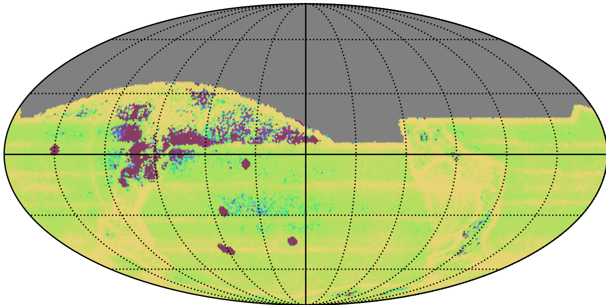
too_elab_r32_d2_griz_v3.4_10yrs All sky: Median Intra-Night Gap
