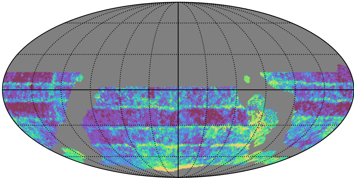
too_elab_r32_d2_griz_v3.4_10yrs WFD r band: Median Inter-Night Gap
