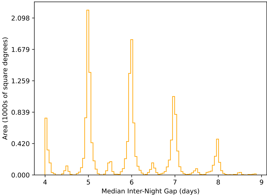
too_elab_r32_d2_griz_v3.4_10yrs WFD r band: Median Inter-Night Gap
