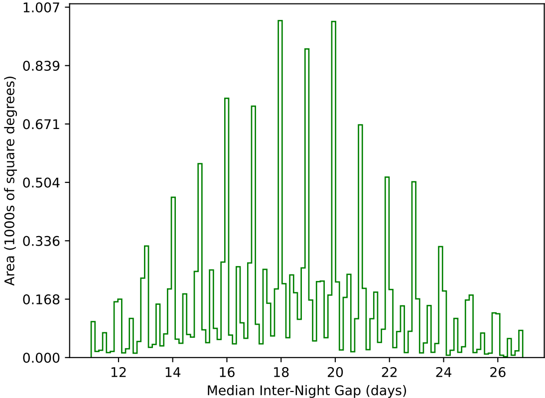
too_elab_r32_d2_griz_v3.4_10yrs WFD g band: Median Inter-Night Gap
