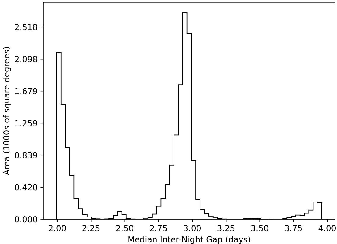
too_elab_r32_d2_griz_v3.4_10yrs WFD all bands: Median Inter-Night Gap
