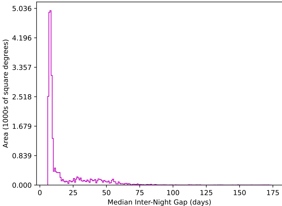
too_elab_r32_d2_griz_v3.4_10yrs All sky z band: Median Inter-Night Gap
