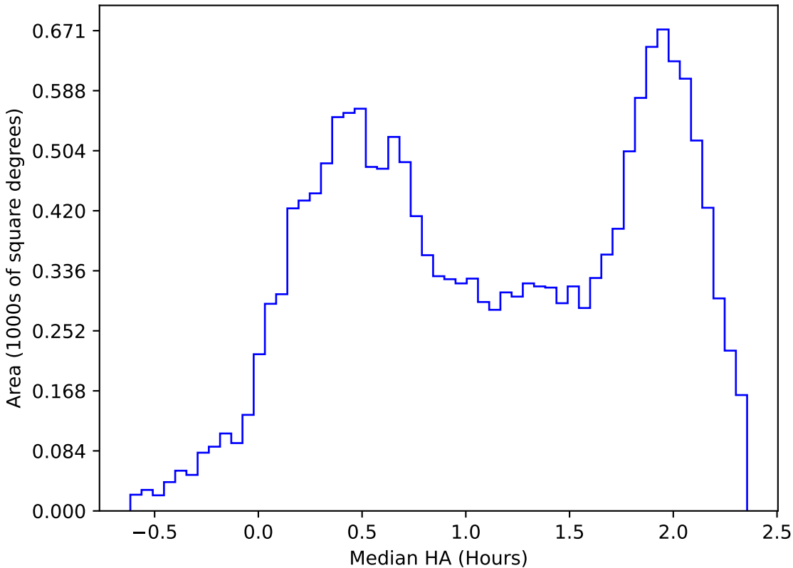
too_elab_r32_d2_griz_v3.4_10yrs WFD z band: Median HA
