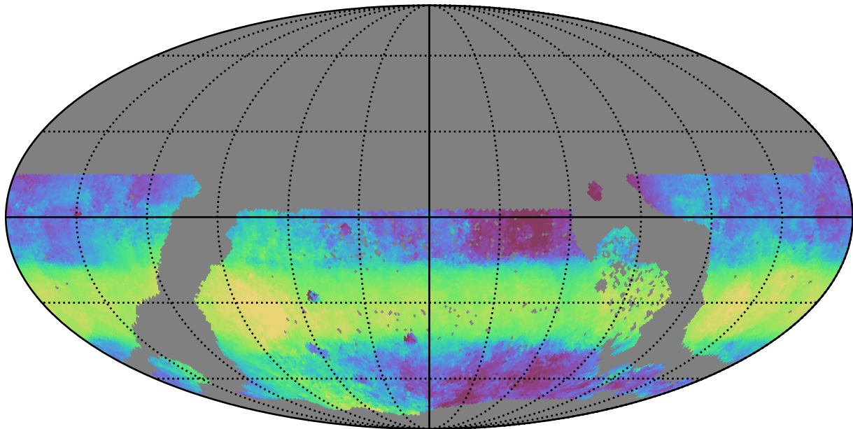
too_elab_r32_d2_griz_v3.4_10yrs WFD y band: Median HA
