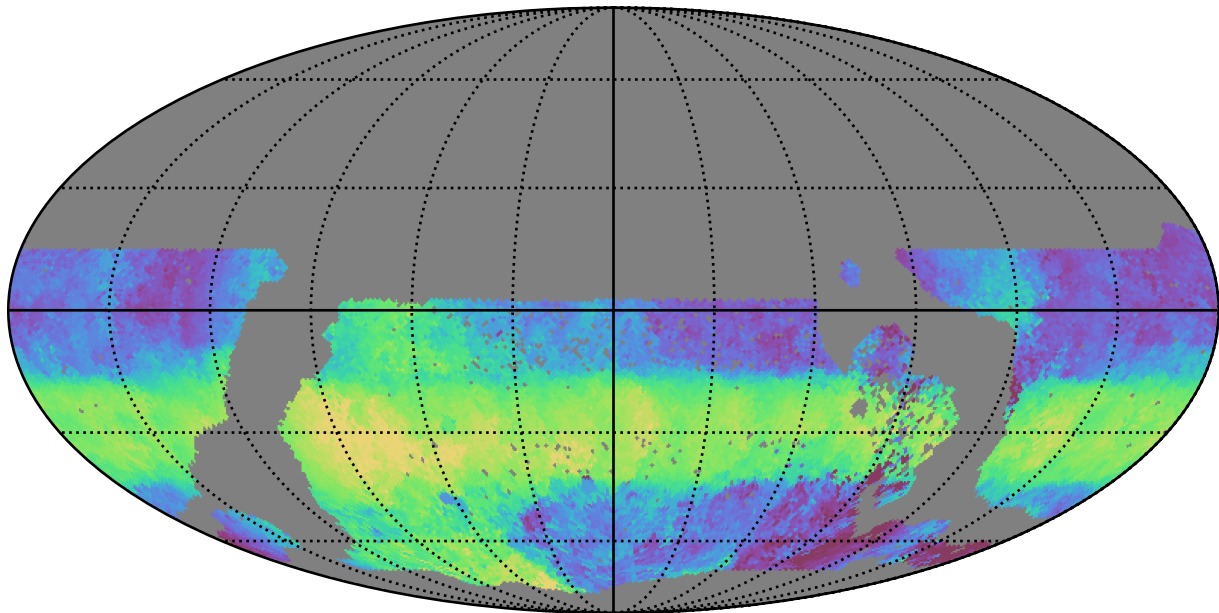
too_elab_r32_d2_griz_v3.4_10yrs WFD u band: Median HA
