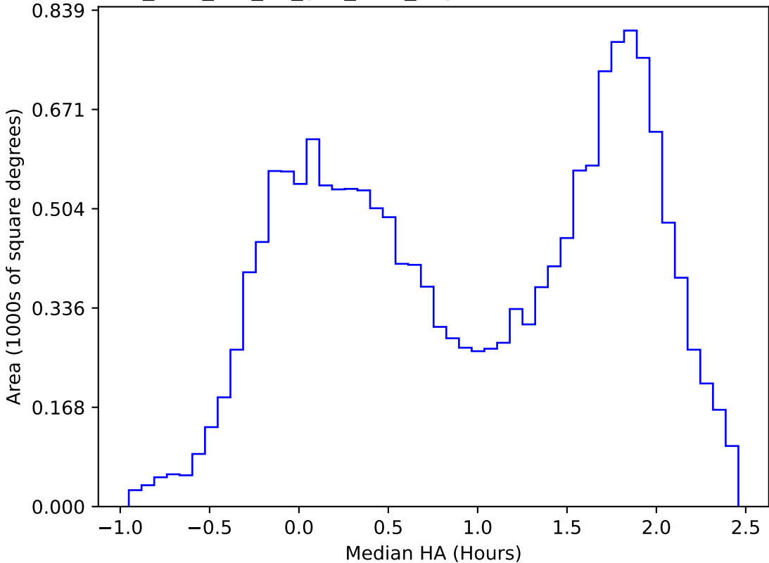
too_elab_r32_d2_griz_v3.4_10yrs WFD u band: Median HA
