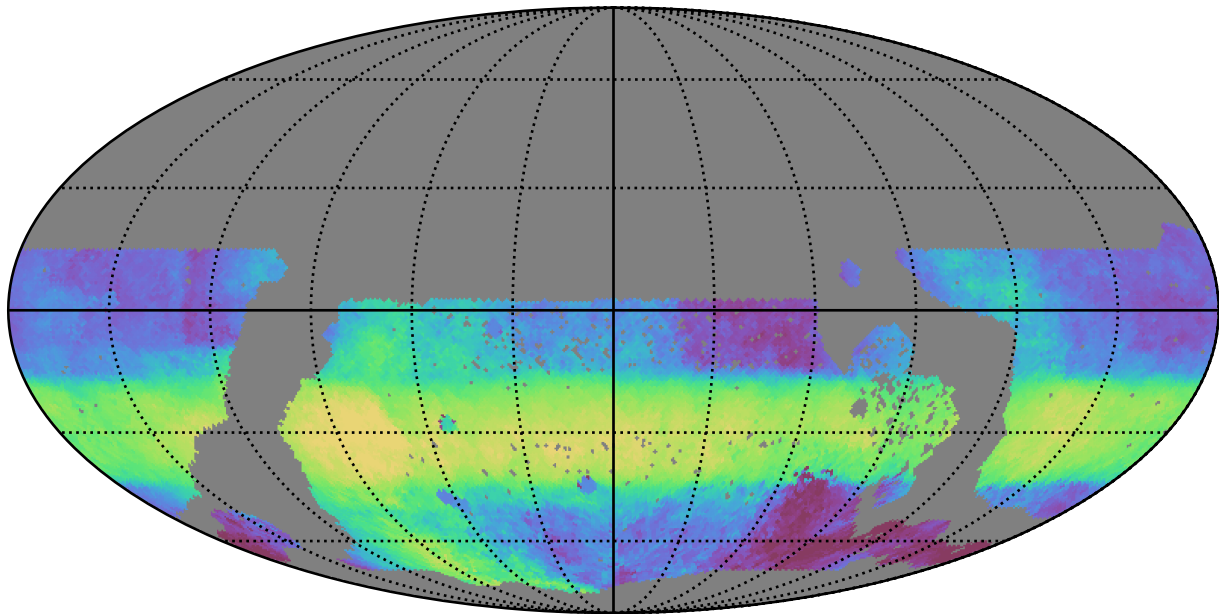
too_elab_r32_d2_griz_v3.4_10yrs WFD r band: Median HA
