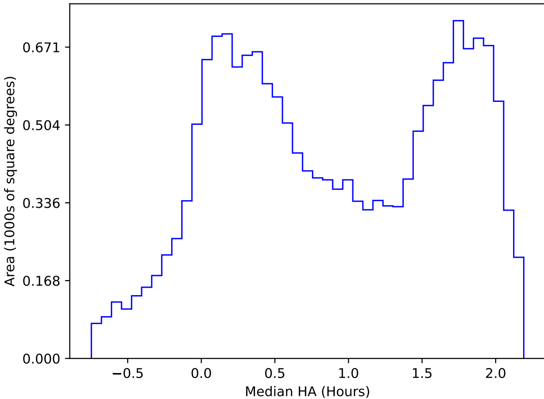
too_elab_r32_d2_griz_v3.4_10yrs WFD r band: Median HA
