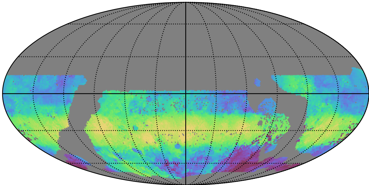
too_elab_r32_d2_griz_v3.4_10yrs WFD g band: Median HA
