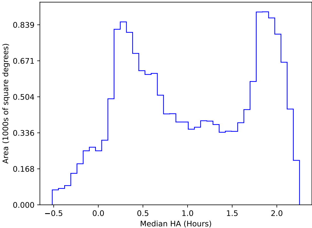
too_elab_r32_d2_griz_v3.4_10yrs WFD all bands: Median HA
