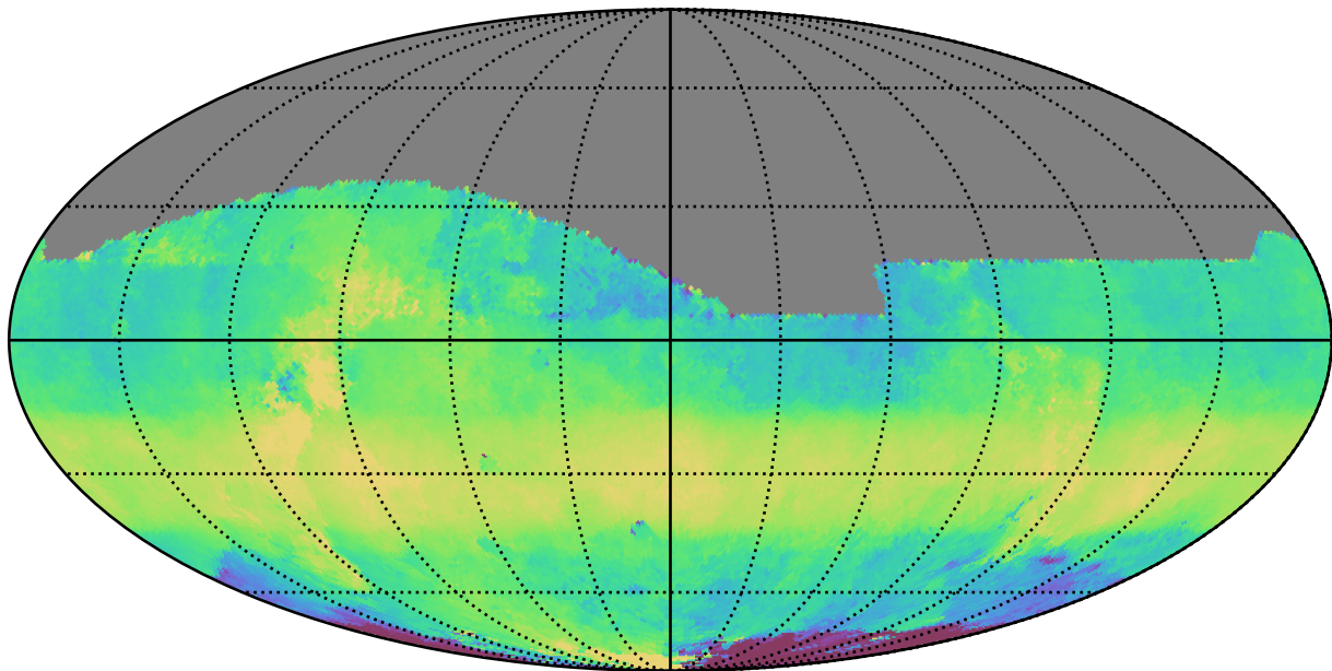
too_elab_r32_d2_griz_v3.4_10yrs All sky z band: Median HA
