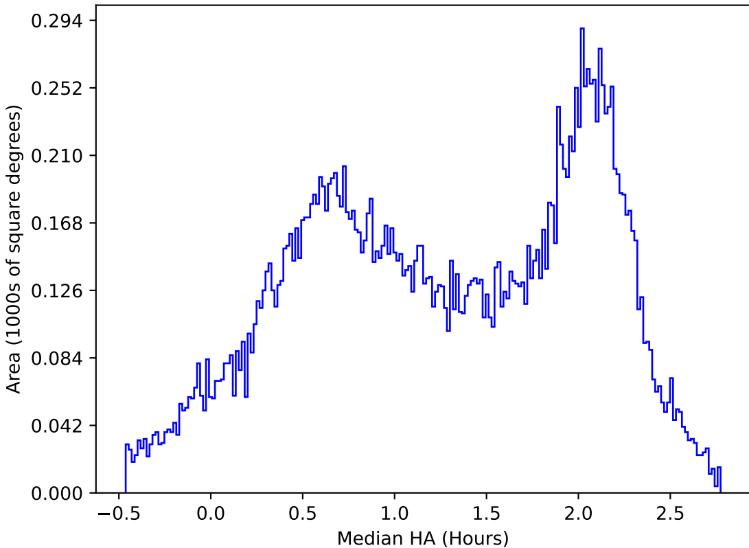
too_elab_r32_d2_griz_v3.4_10yrs All sky y band: Median HA
