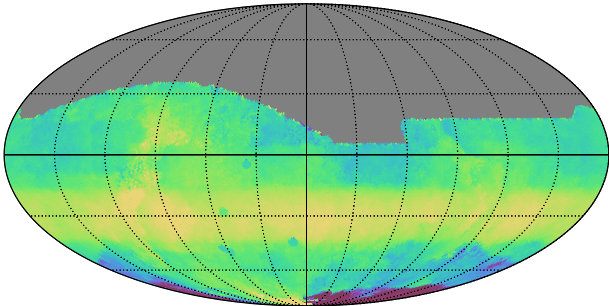
too_elab_r32_d2_griz_v3.4_10yrs All sky i band: Median HA
