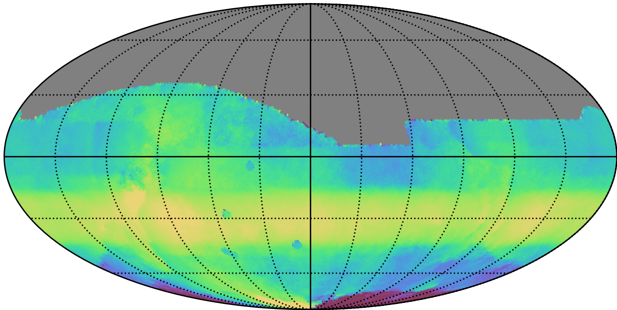
too_elab_r32_d2_griz_v3.4_10yrs All sky all bands: Median HA
