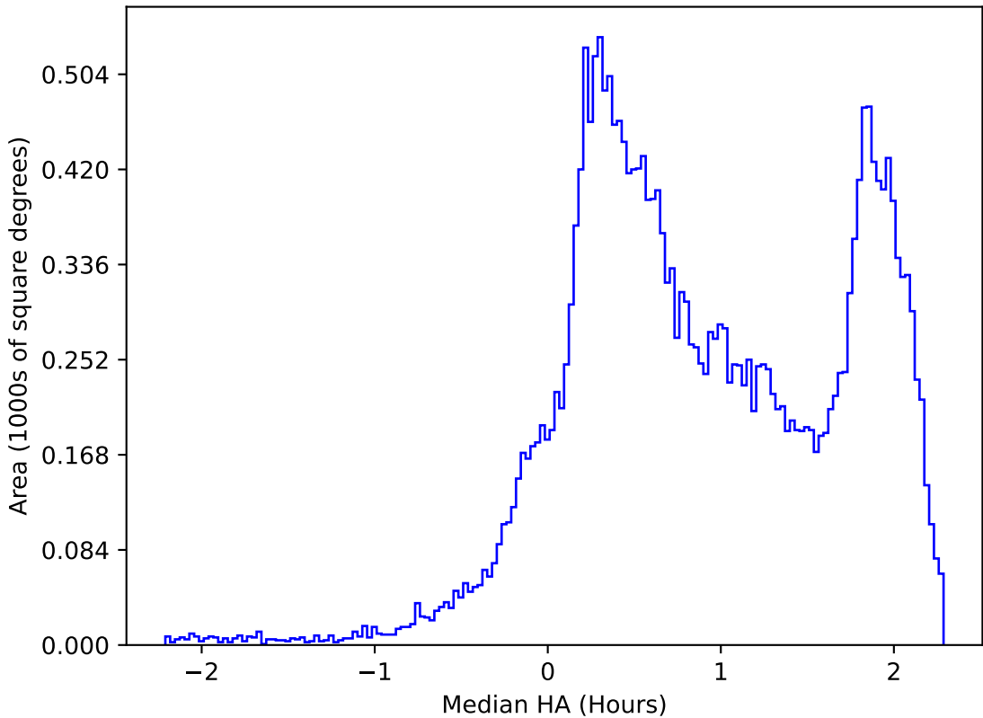
too_elab_r32_d2_griz_v3.4_10yrs All sky all bands: Median HA
