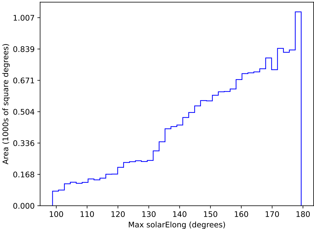
too_elab_r32_d2_griz_v3.4_10yrs WFD z band: Max solarElong
