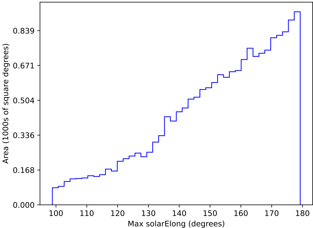
too_elab_r32_d2_griz_v3.4_10yrs WFD y band: Max solarElong
