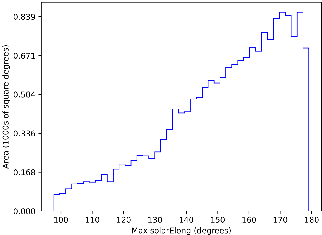
too_elab_r32_d2_griz_v3.4_10yrs WFD u band: Max solarElong
