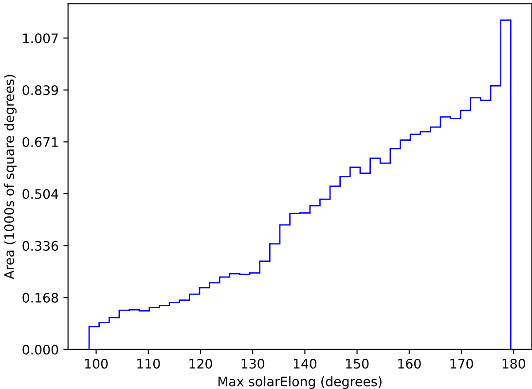
too_elab_r32_d2_griz_v3.4_10yrs WFD i band: Max solarElong
