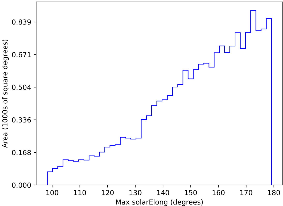
too_elab_r32_d2_griz_v3.4_10yrs WFD g band: Max solarElong
