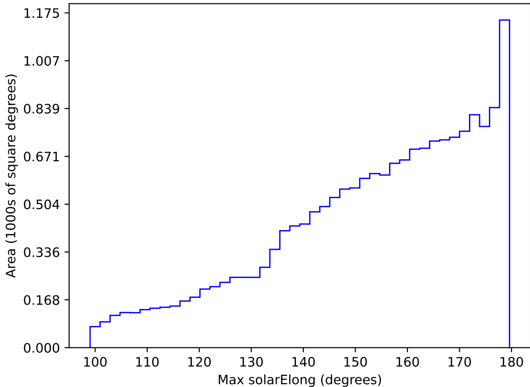
too_elab_r32_d2_griz_v3.4_10yrs WFD all bands: Max solarElong
