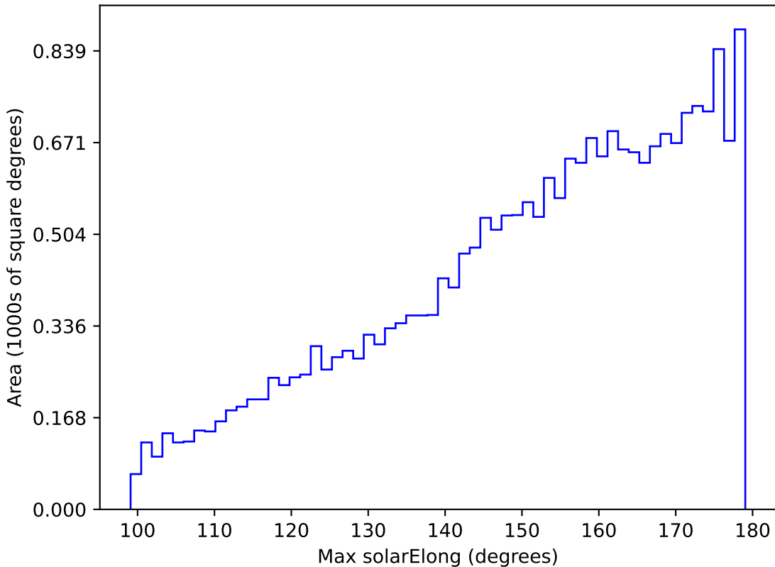
too_elab_r32_d2_griz_v3.4_10yrs All sky y band: Max solarElong
