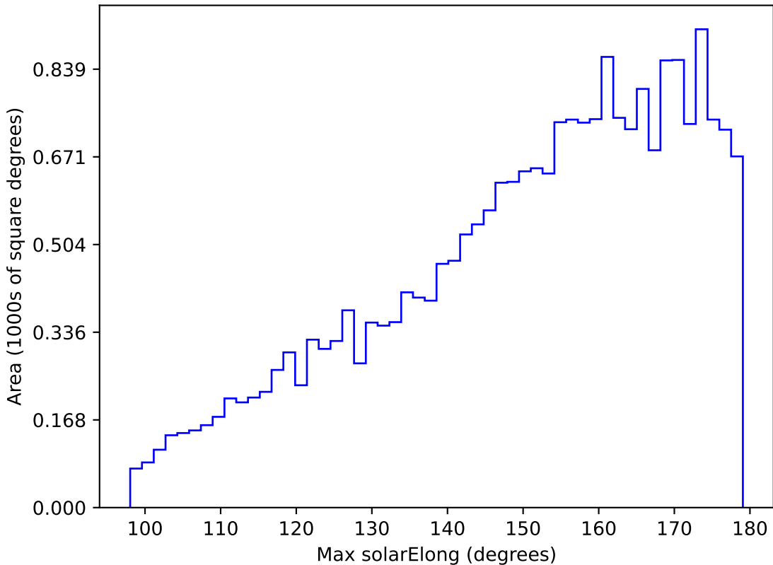
too_elab_r32_d2_griz_v3.4_10yrs All sky u band: Max solarElong
