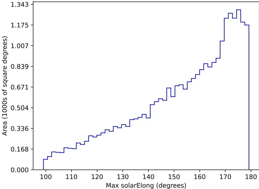
too_elab_r32_d2_griz_v3.4_10yrs All sky g band: Max solarElong
