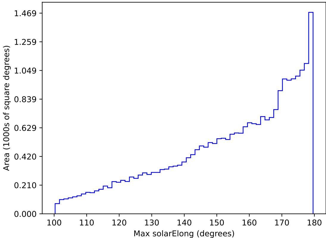
too_elab_r32_d2_griz_v3.4_10yrs All sky all bands: Max solarElong
