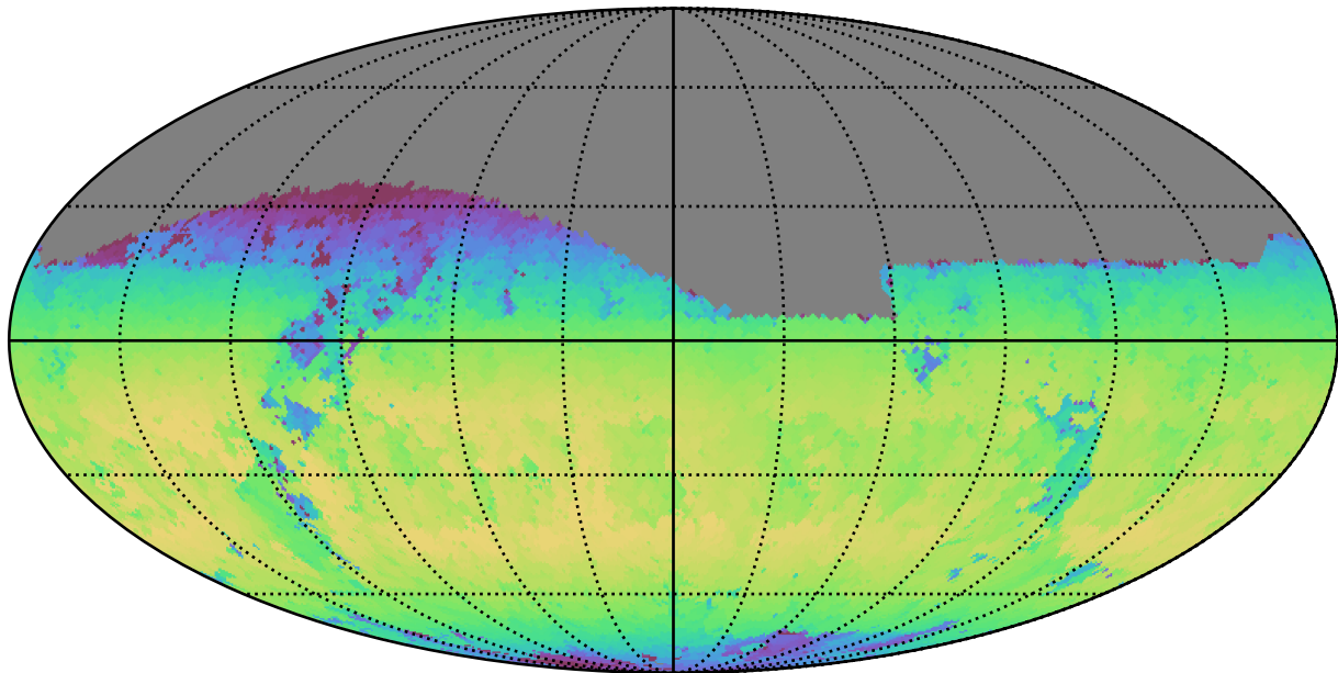
too_elab_r32_d2_griz_v3.4_10yrs Yr 1 z band: Max skyBrightness
