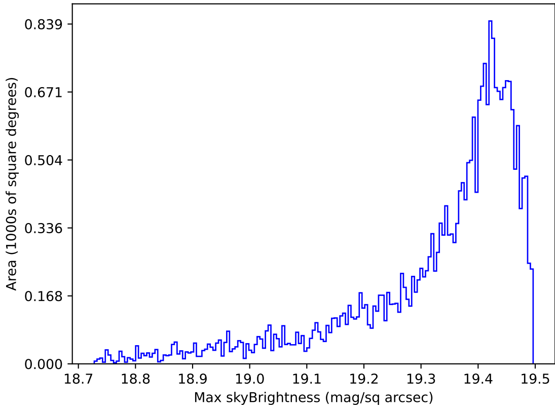
too_elab_r32_d2_griz_v3.4_10yrs Yr 1 z band: Max skyBrightness
