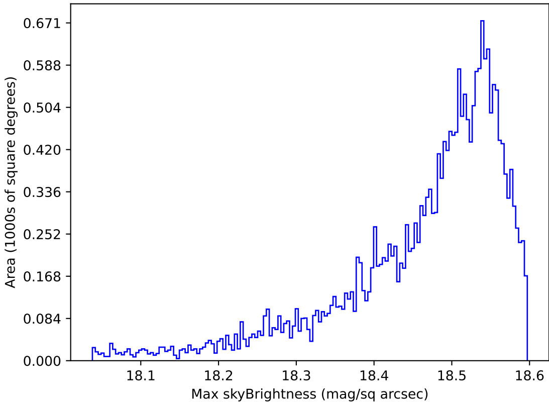
too_elab_r32_d2_griz_v3.4_10yrs Yr 1 y band: Max skyBrightness
