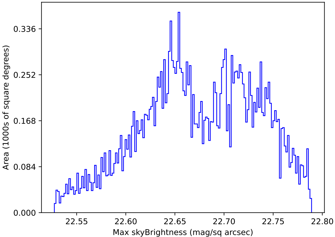
too_elab_r32_d2_griz_v3.4_10yrs Yr 1 u band: Max skyBrightness
