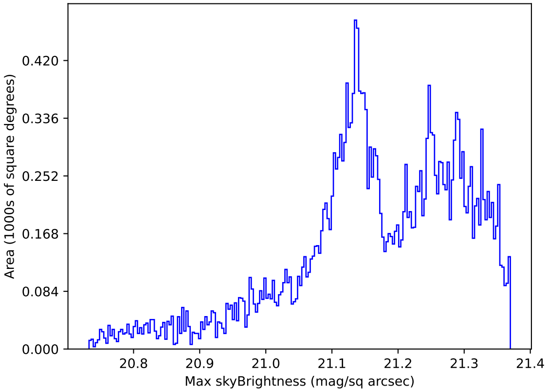
too_elab_r32_d2_griz_v3.4_10yrs Yr 1 r band: Max skyBrightness
