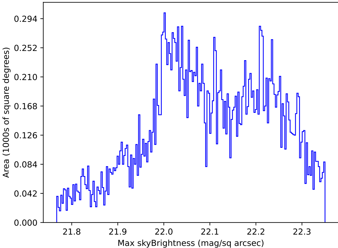
too_elab_r32_d2_griz_v3.4_10yrs Yr 1 g band: Max skyBrightness
