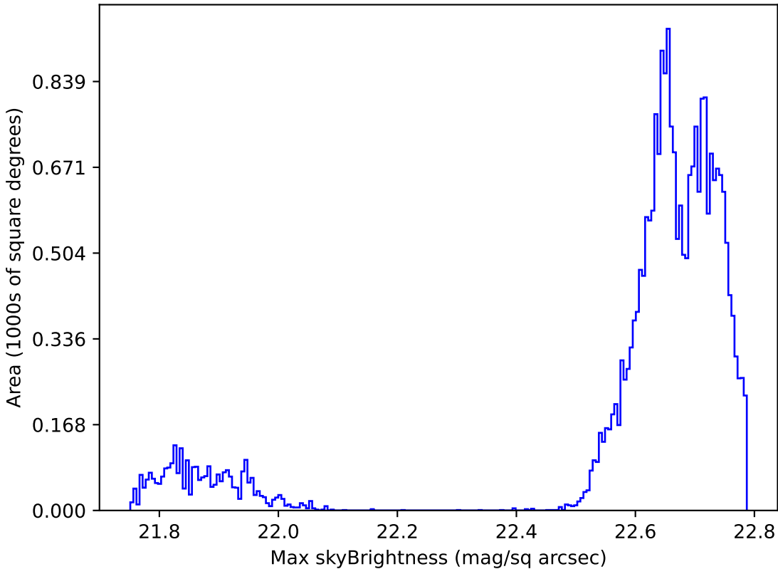
too_elab_r32_d2_griz_v3.4_10yrs Yr 1 all bands: Max skyBrightness
