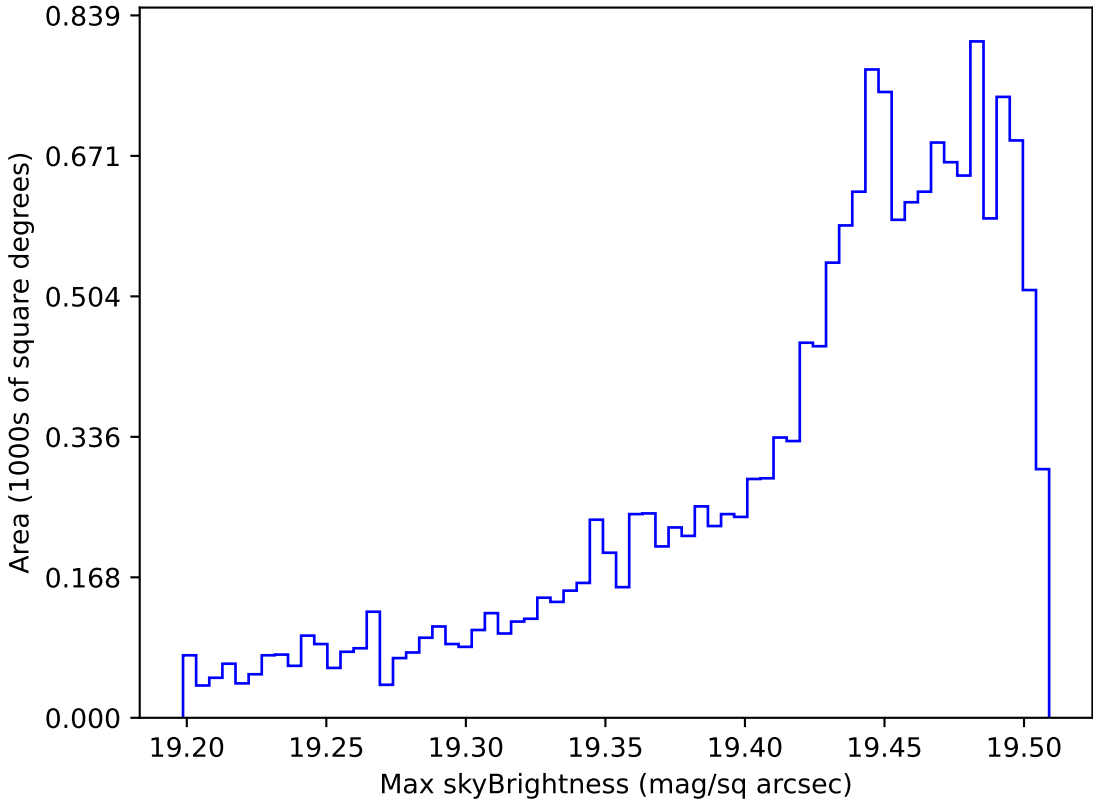
too_elab_r32_d2_griz_v3.4_10yrs WFD z band: Max skyBrightness
