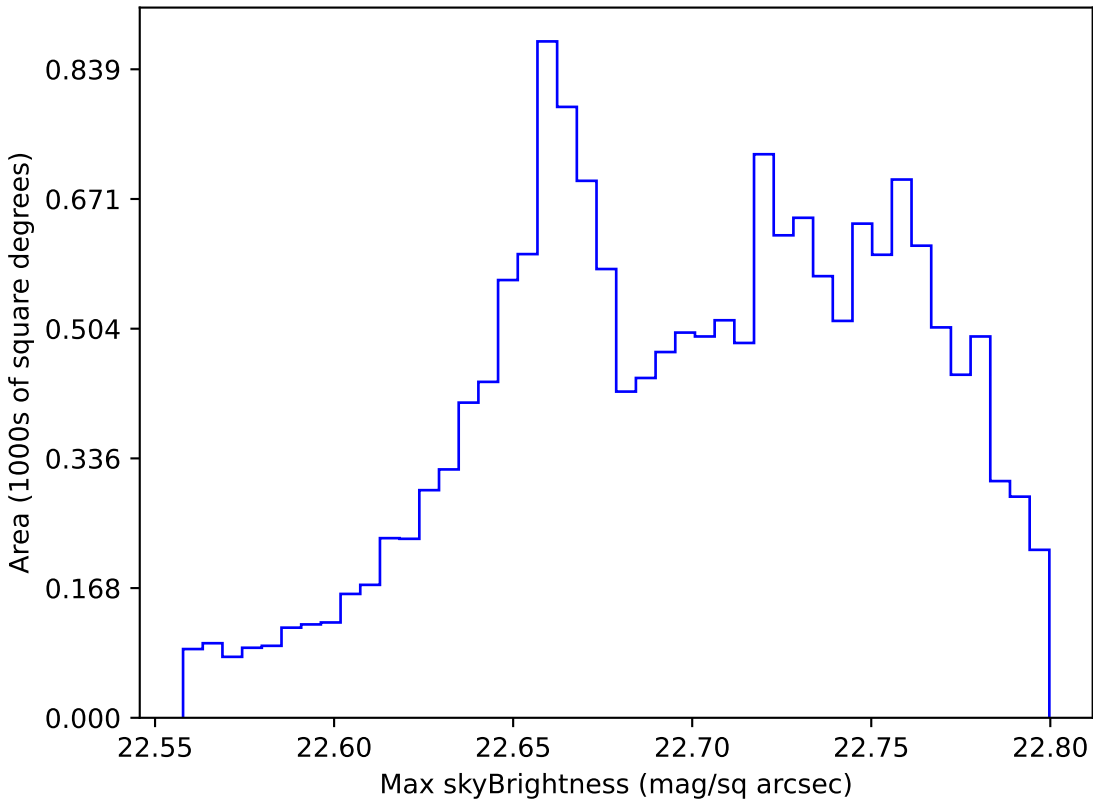
too_elab_r32_d2_griz_v3.4_10yrs WFD u band: Max skyBrightness
