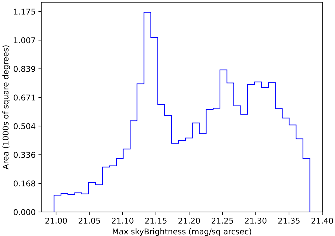
too_elab_r32_d2_griz_v3.4_10yrs WFD r band: Max skyBrightness
