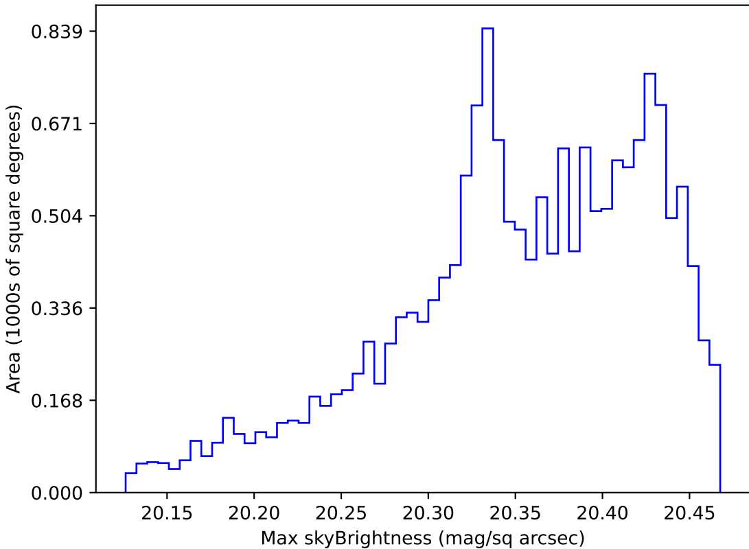
too_elab_r32_d2_griz_v3.4_10yrs WFD i band: Max skyBrightness
