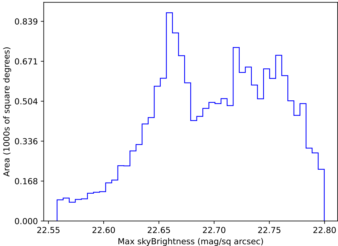
too_elab_r32_d2_griz_v3.4_10yrs WFD all bands: Max skyBrightness
