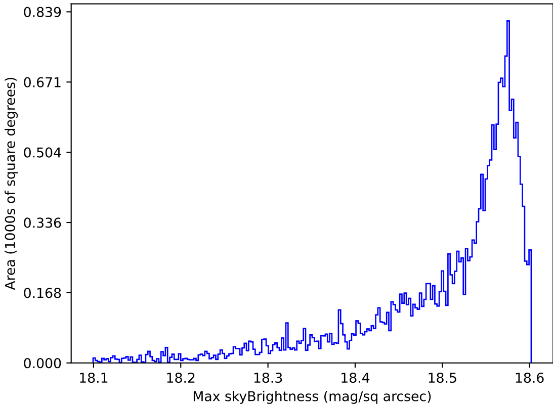
too_elab_r32_d2_griz_v3.4_10yrs All sky y band: Max skyBrightness
