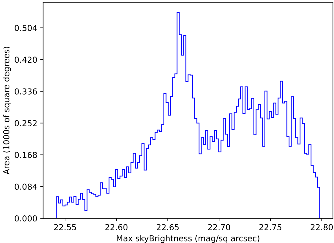
too_elab_r32_d2_griz_v3.4_10yrs All sky u band: Max skyBrightness
