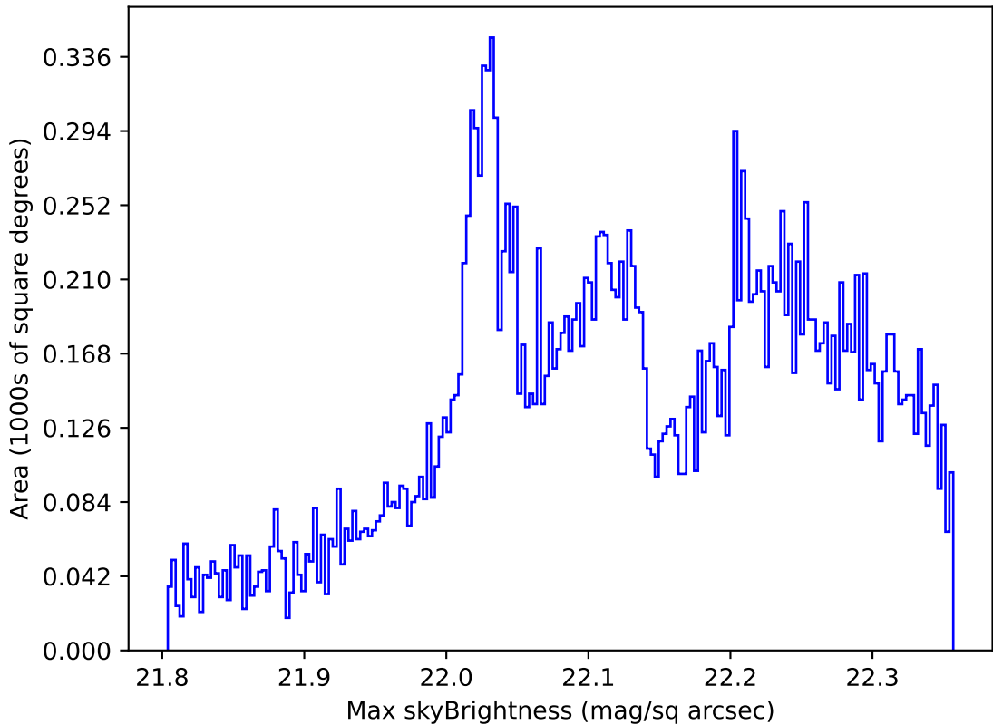
too_elab_r32_d2_griz_v3.4_10yrs All sky g band: Max skyBrightness
