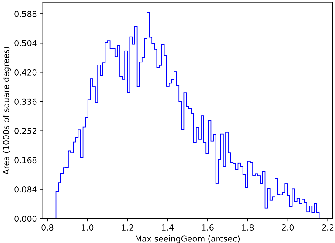
too_elab_r32_d2_griz_v3.4_10yrs Yr 1 r band: Max seeingGeom
