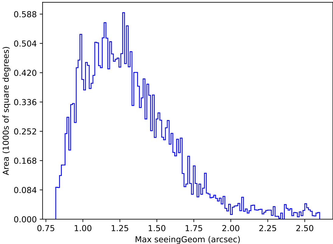
too_elab_r32_d2_griz_v3.4_10yrs Yr 1 i band: Max seeingGeom
