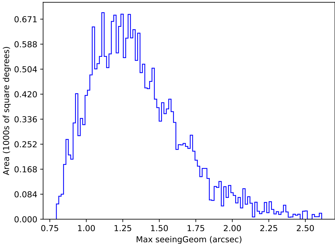
too_elab_r32_d2_griz_v3.4_10yrs Yr 1 g band: Max seeingGeom
