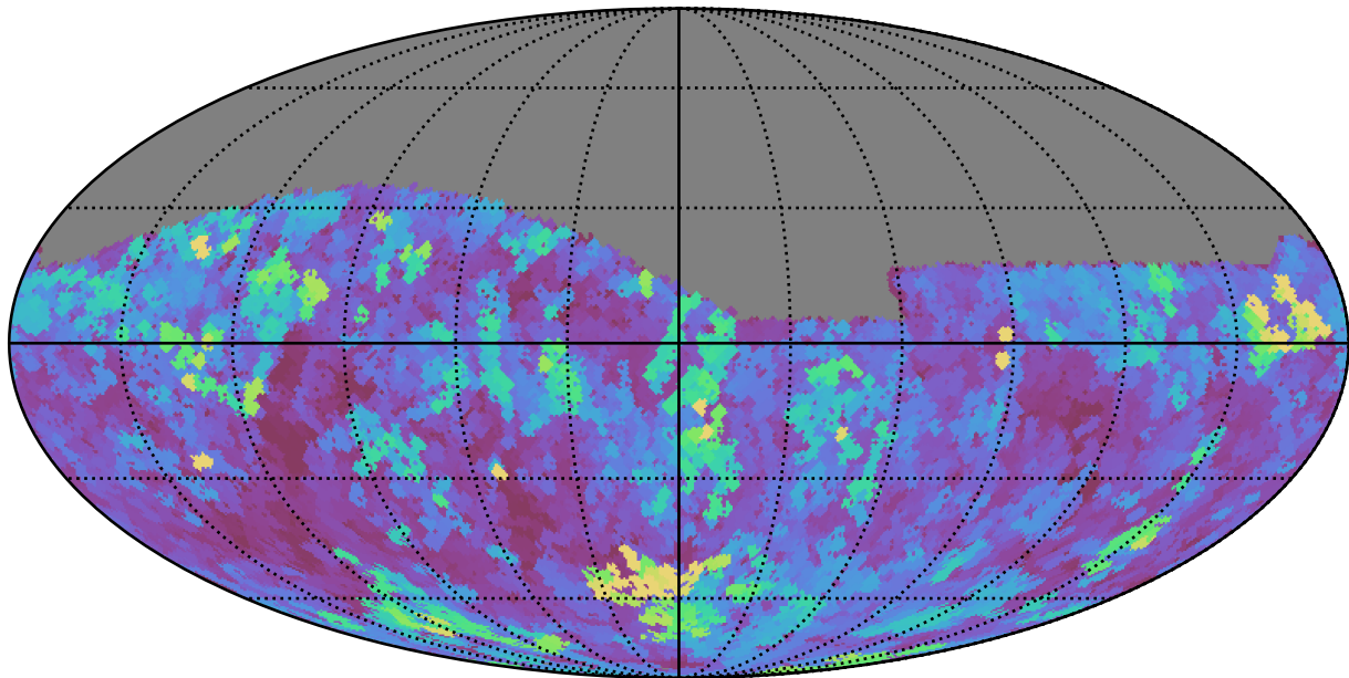
too_elab_r32_d2_griz_v3.4_10yrs Yr 1 z band: Max seeingEff
