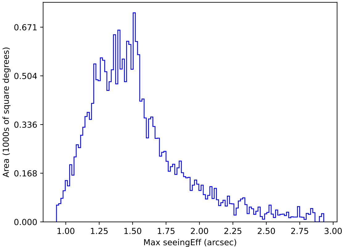
too_elab_r32_d2_griz_v3.4_10yrs Yr 1 y band: Max seeingEff
